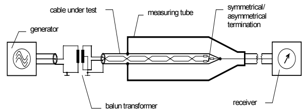
Fig. 18: test set-up for the determination of the coupled power attenuation of a shielded twisted pair.
