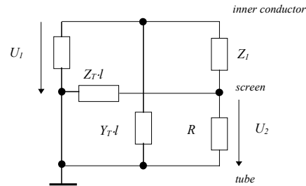
Fig. 4: Equivalent circuit of the triaxial measuring set-up
