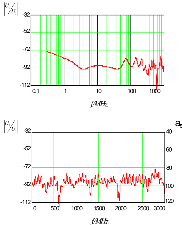
Fig. 13: Frequency response of logarithmic voltage ratio |U_2/U_1| in dB (left hand scale) and screening attenuation a_s (right hand scale) of double braid screen, Cable Type RG 223, coupling length l = 2 m
