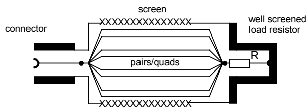
Fig. 17: preparation of symmetrical multi pair/quad cables
