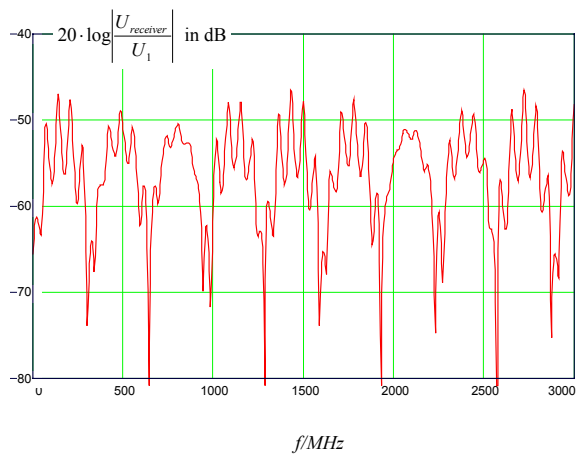
Fig. 16: calculated voltage ratio including multiple reflections caused by the screening case, quantities used:
