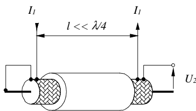
Fig. 1: Definition of transfer impedance
