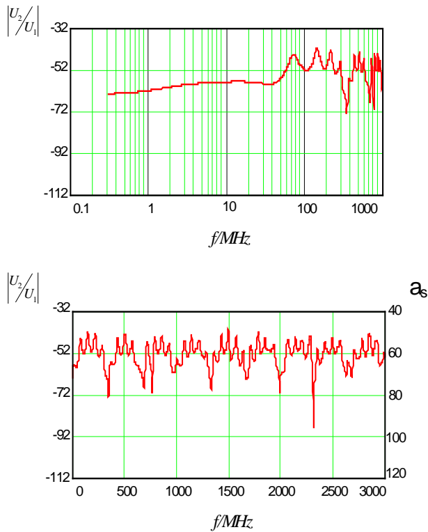
Fig. 9: Frequency response of logarithmic voltage ratio |U_2/U_1| in dB (left hand scale) and screening attenuation a_s (right hand scale) of single braid screen, Cable Type RG 58, coupling length l = 2 m
