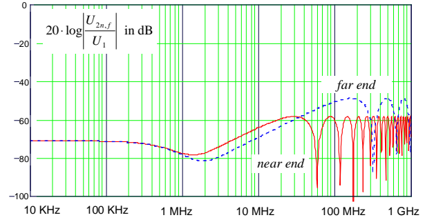
Fig. 5.: calculated voltage ratio for a typical braided cable screen, quantities used:
