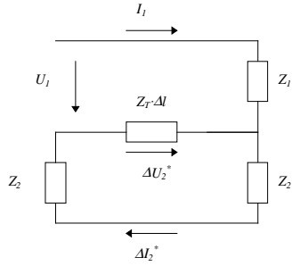
Fig. 8 Equivalent circuit for an electrical short part of the length \Delta l and negligible capacitive coupling
