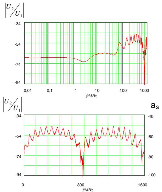
Fig. 12: Frequency response of logarithmic voltage ratio |U_2/U_1| in dB (left hand scale) and screening attenuation a_s (right hand scale) of Cable Type HF 75 1,0/4,8 02YCY, \epsilon_{r1}=1,7 , |\Delta v/v_1| = 24\% , coupling length l = 2 m
