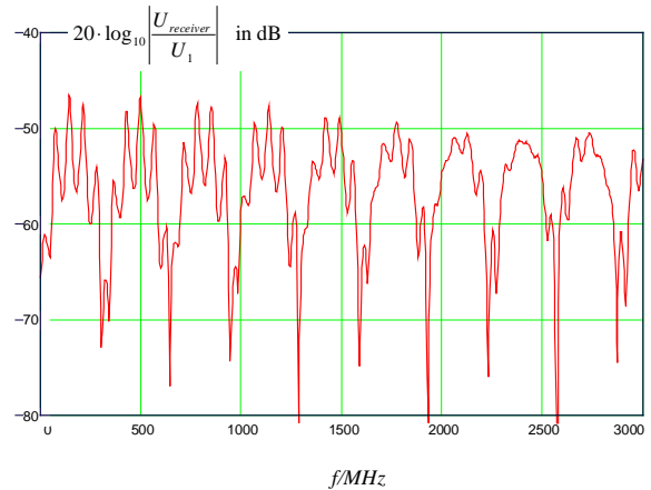
Fig. 15: calculated voltage ratio including multiple reflections caused by the screening case, quantities used:
