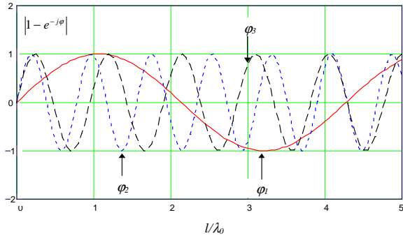
Fig. 6.: calculated periodic functions for \epsilon_{r1} = 2,3 and \epsilon_{r2} = 1,1
