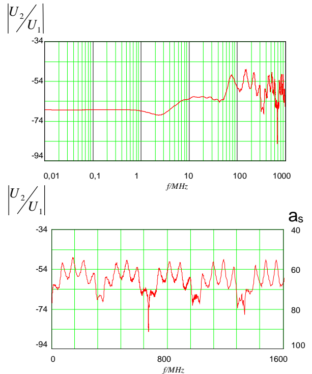
Fig. 11: Frequency response of logarithmic voltage ratio |U_2/U_1| in dB (left hand scale) and screening attenuation a_s (right hand scale) of Cable Type HF 75 0,7/4,8 2YCY, \epsilon_{r1}=2,3 , |\Delta v/v_1| = 45\% , coupling length l = 2 m
