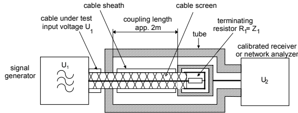
Fig. 3: Triaxial measuring set-up for screening attenuation
