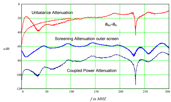
Fig. 19.: EMC of cable type IBM Twinax 105 \Omega
