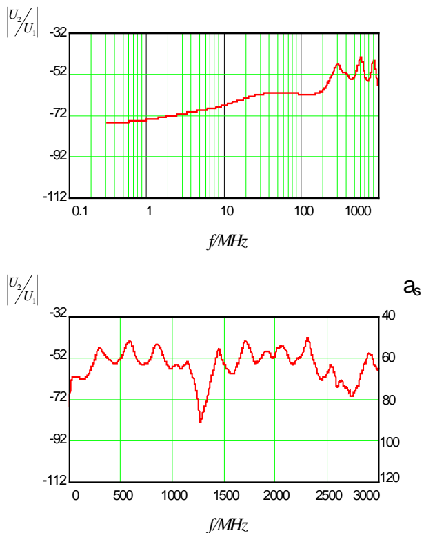
Fig. 10: Frequency response of logarithmic voltage ratio |U_2/U_1| in dB (left hand scale) and screening attenuation a_s (right hand scale) of single braid screen, Cable Type RG 58, coupling length l = 0,5 m
