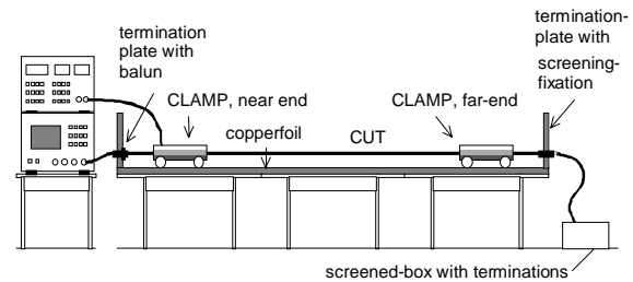
Fig. 9: injection clamp set-up
