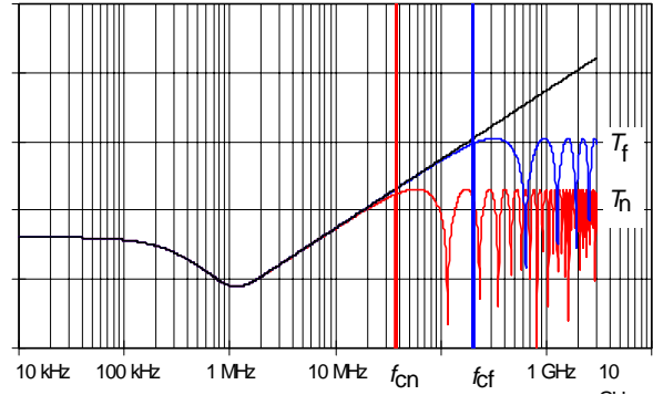
Fig. 3: Calculated coupling transfer function ( l = 1 m; \epsilon_{r1} = 2,3 ; \epsilon_{r2} = 1 ; Z_F = 0 )
