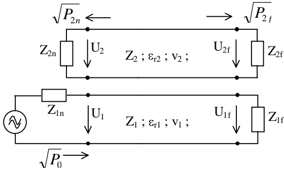
Fig. 1: Equivalent circuit
