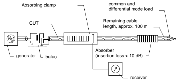
Fig. 8: Test set-up for the coupling attenuation absorbing clamp method
