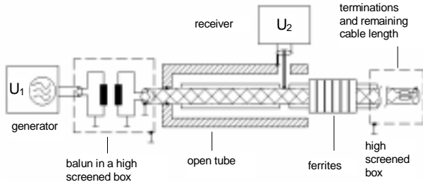
Fig. 10: Triaxial set-up to measure the coupling attenuation
